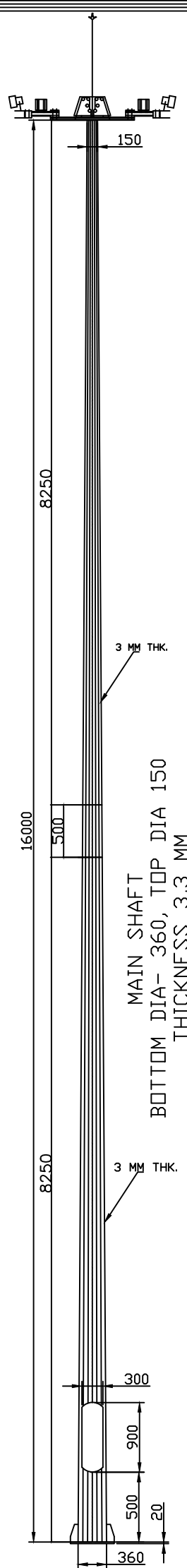
16 MTR HIGH MAST POLE WITH 8 LUMINAARIES
