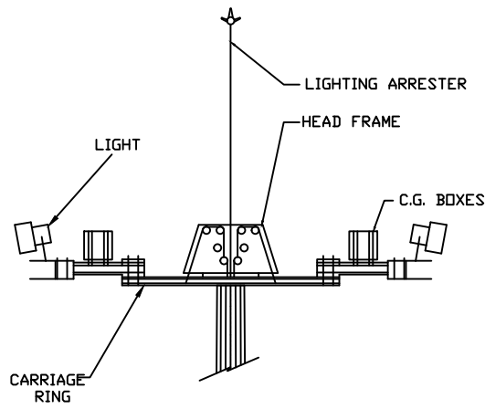
DISTRIBUTION OF LUMINARIES
