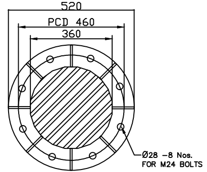
BASE PLATE DIA 520X20 MM THK.
